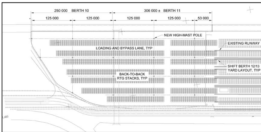
Figure 3. Berths 10 and 11 container yard layout.
