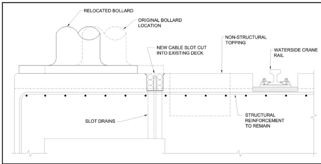
Figure 7. Waterside crane cable relocation detail.
