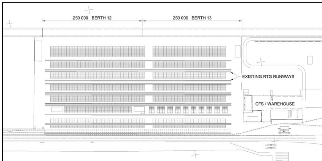
Figure 2. Berths 12 and 13 container yard layout.
