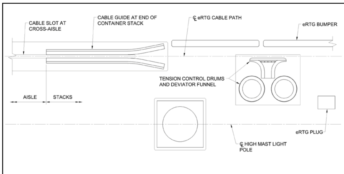
Figure 5. eRTG plug and cabling layout.
