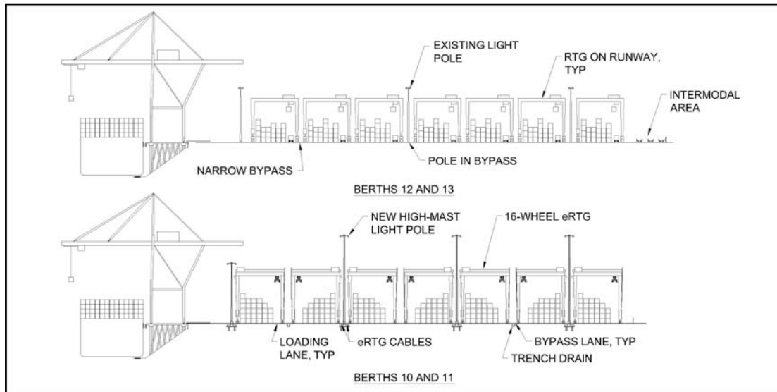
Figure 4. Comparison of berths container yard sections.
