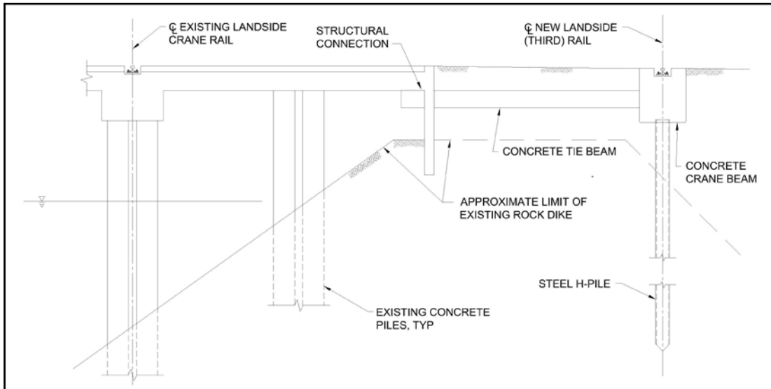
Figure 6. General arrangement of third rail and new/existing cranes.
