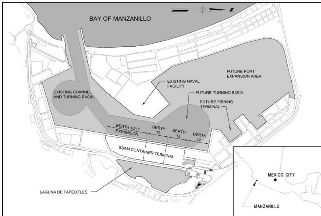
Figure 1. Site plan.
